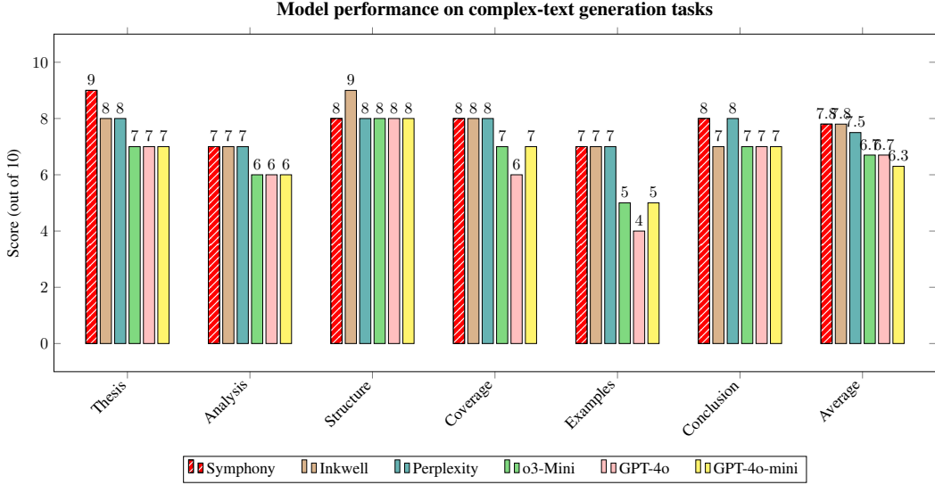
Figure 3: Performance of models and agents across evaluation dimensions
